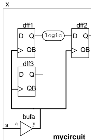
Figure 27: Period constraint
