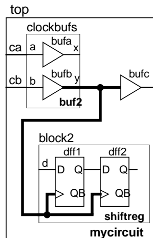
Figure 29: Skew constraint
