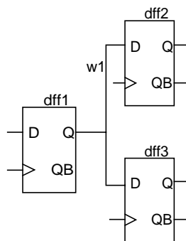
Figure 12: Net Delay
