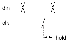
Figure 16: Hold time
