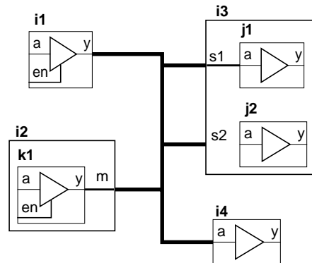
Figure 11: Interconnect delay
