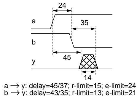
Figure 6: 2-input AND
