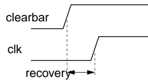
Figure 18: Recovery time
