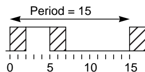
Figure 30: Specification of a waveform of period 15
