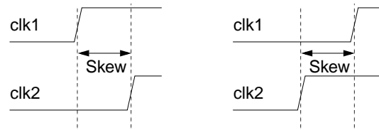
Figure 22: Skew timing check
