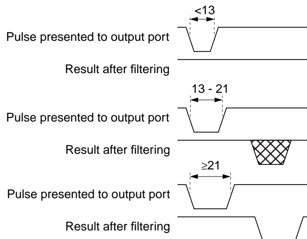
Figure 5: Pulse filtering
