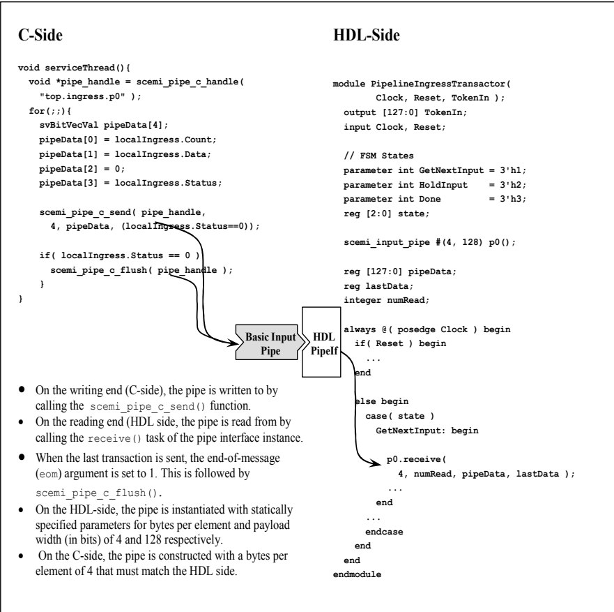
Figure 4.11 Example of Input Pipe
