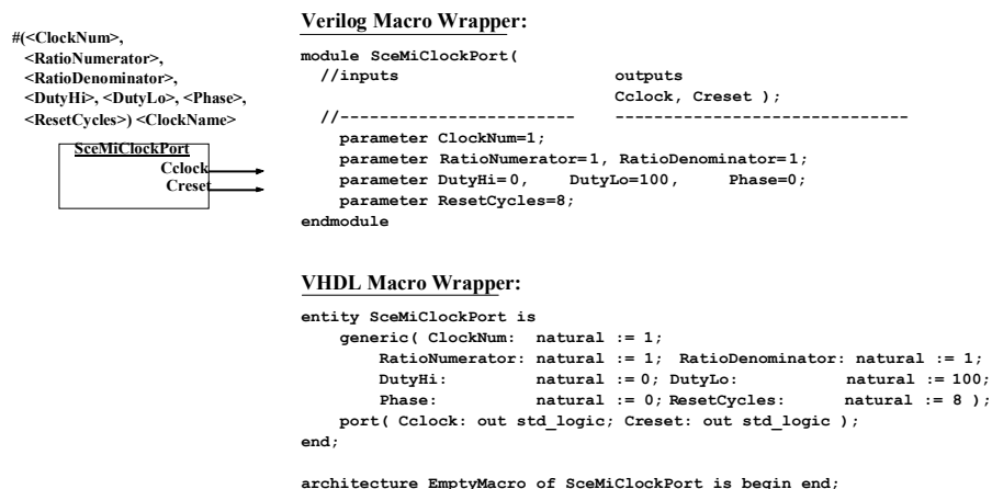
Figure 5.5 SceMiClockPort macro
