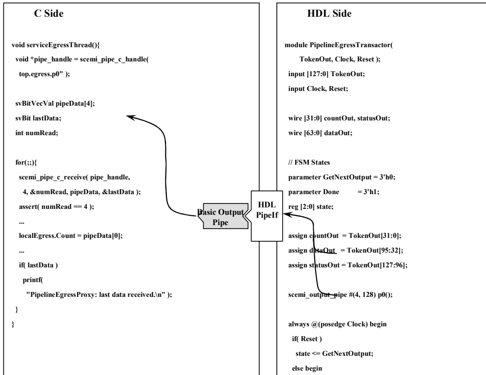
Figure 4.12 Example of output pipe
