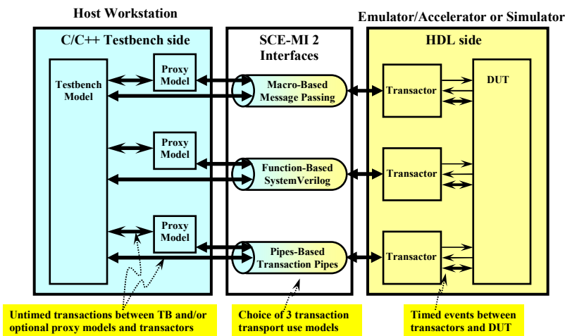
Figure 4.1 Three Interfaces
