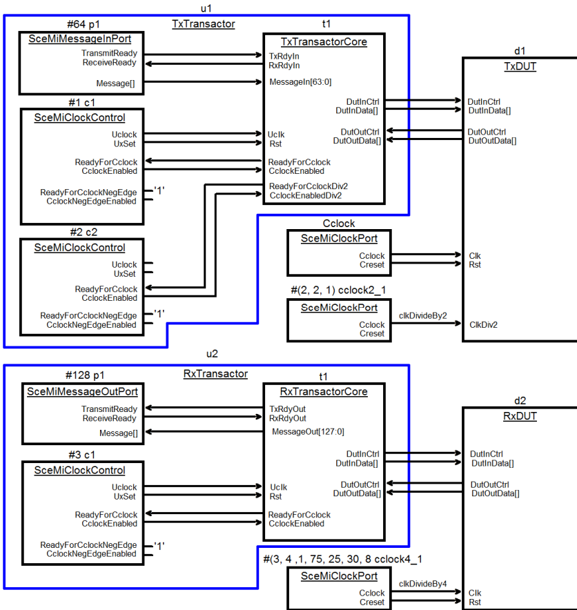
Figure C.1 Multi-clock, multi-transactor example
