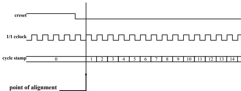
Figure 5.10 Cycle Stamps
