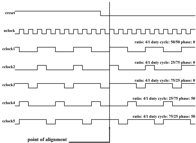
Figure 5.6 Multi-clock alignment
