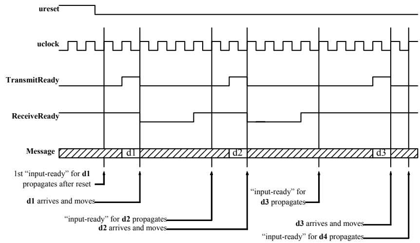
Figure 5.3 SceMiMessageInPort handshake waveforms with input-ready propagation
