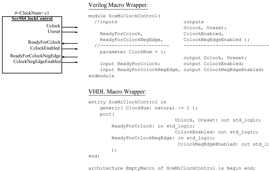
Figure 5.7 SceMiClockControl macro
