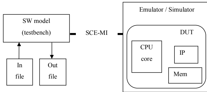
Figure 3.3 Modeling a DUT via an abstraction bridge
