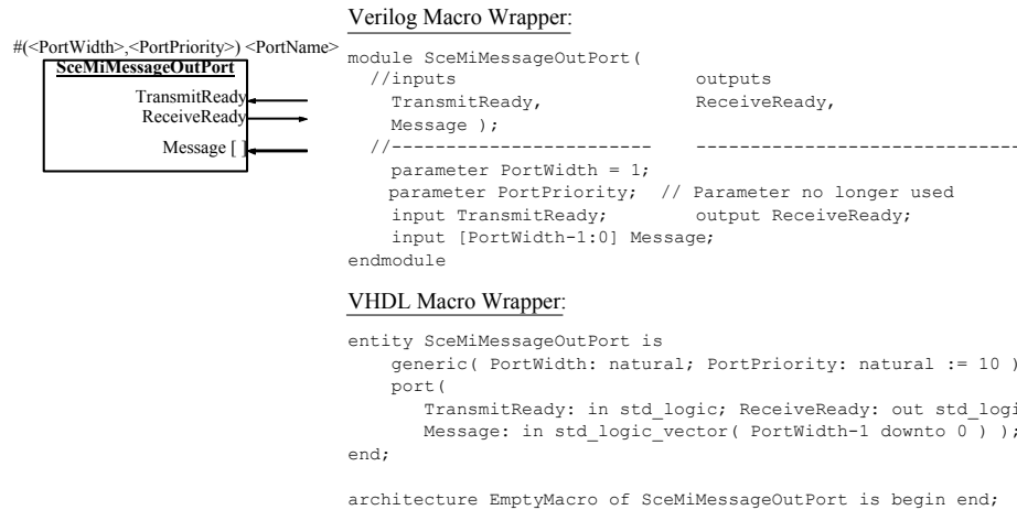
Figure 5.4 SceMiMessageOutPort macro
