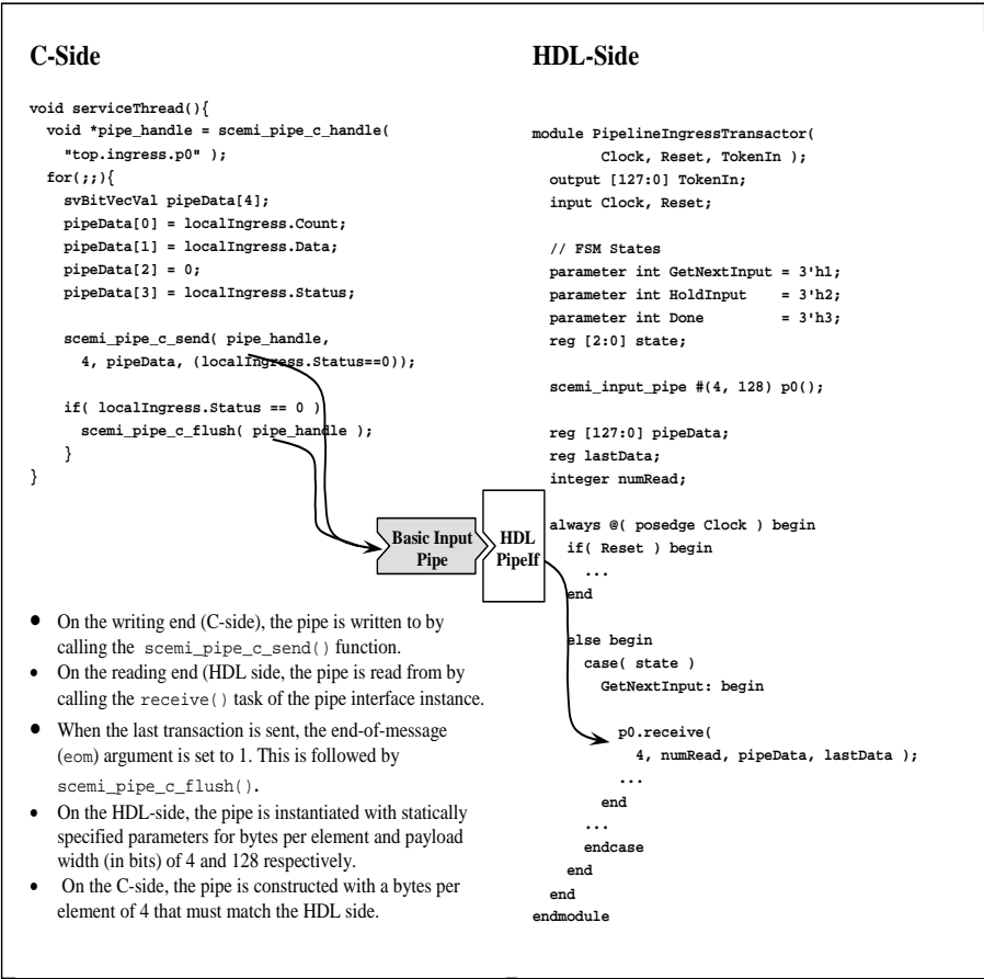
Figure 4.10 Example of Input Pipe
