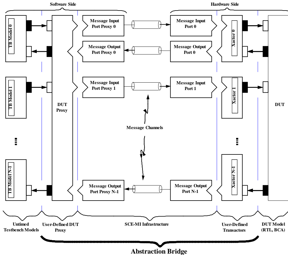
Figure 4.4 Multi-channel abstraction bridge architecture
