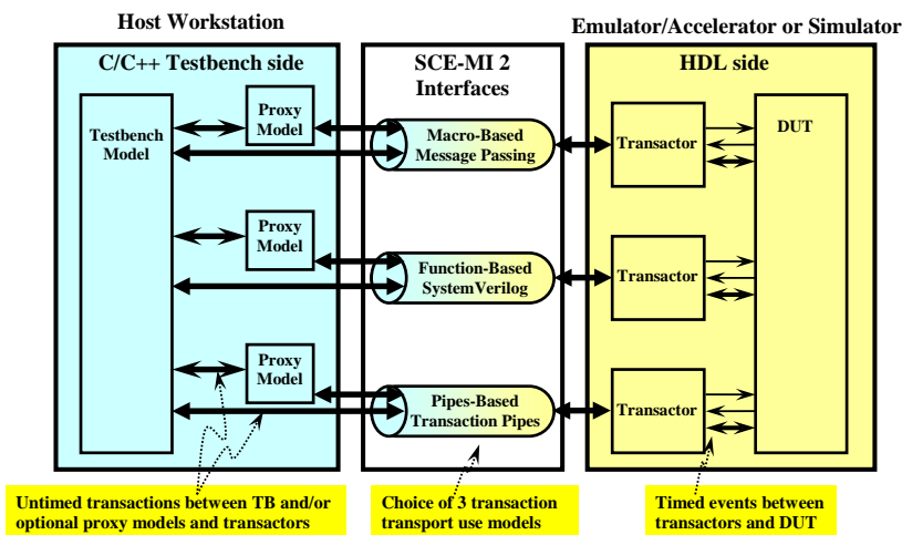
Figure 4.1 Three Interfaces
