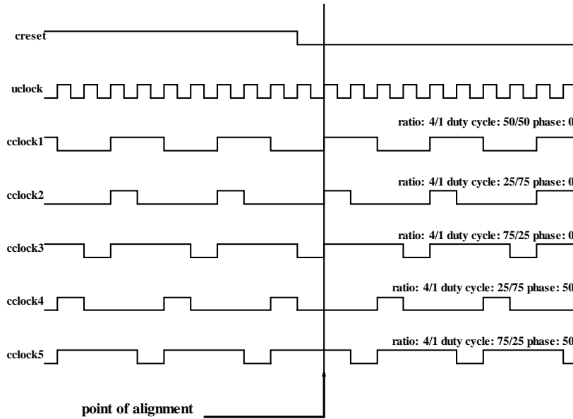
Figure 5.6 Multi-clock alignment
