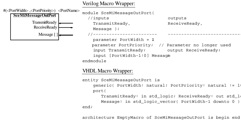
Figure 5.4 SceMiMessageOutPort macro
