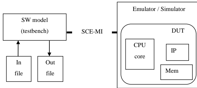
Figure 3.3 Modeling a DUT via an abstraction bridge
