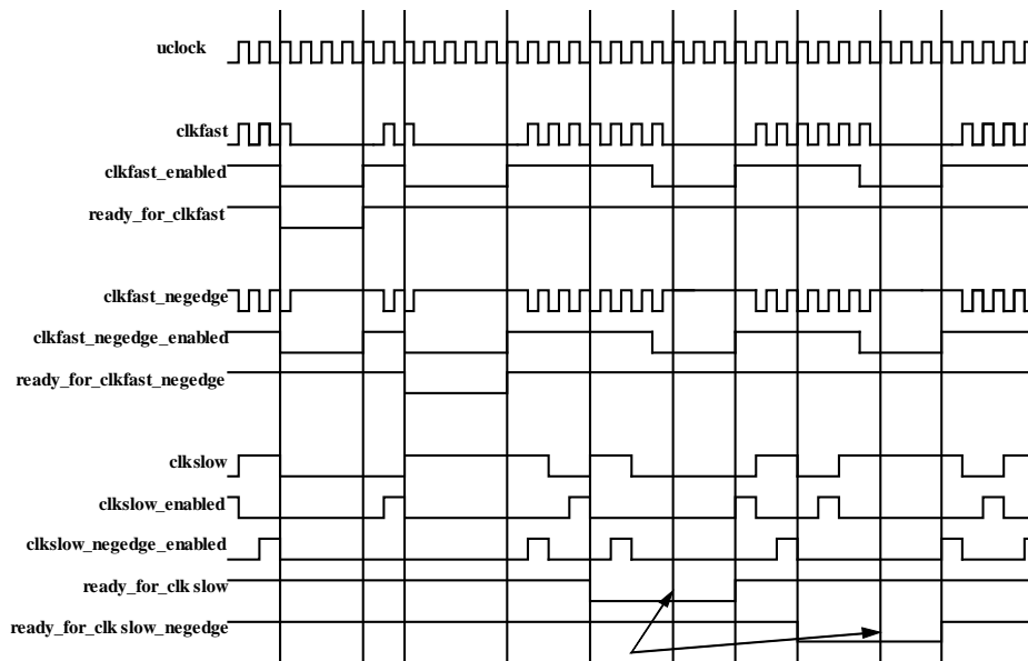
Figure 5.8 Example of Clock Control Semantics
