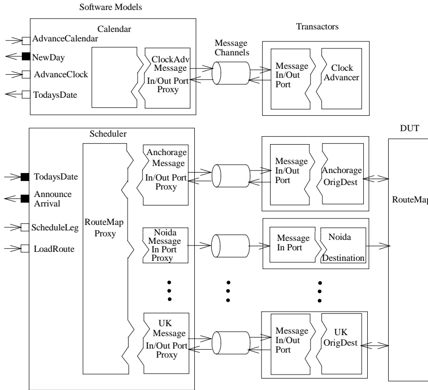
Figure A.3 The bridge
