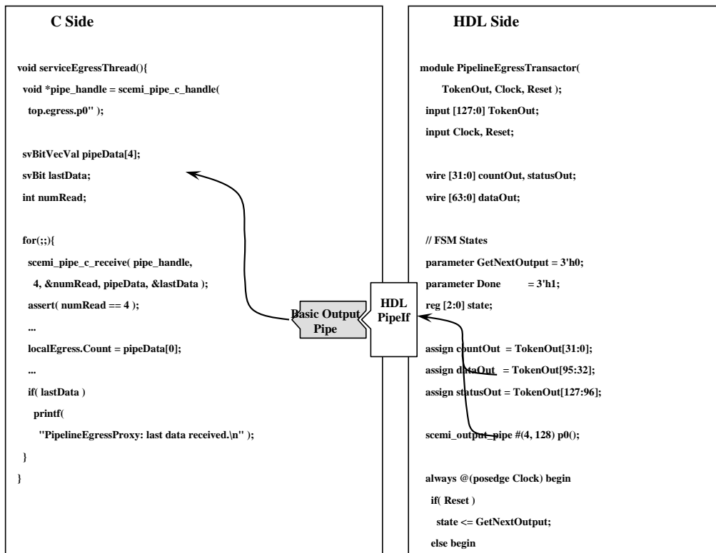
Figure 4.11 Example of output pipe
