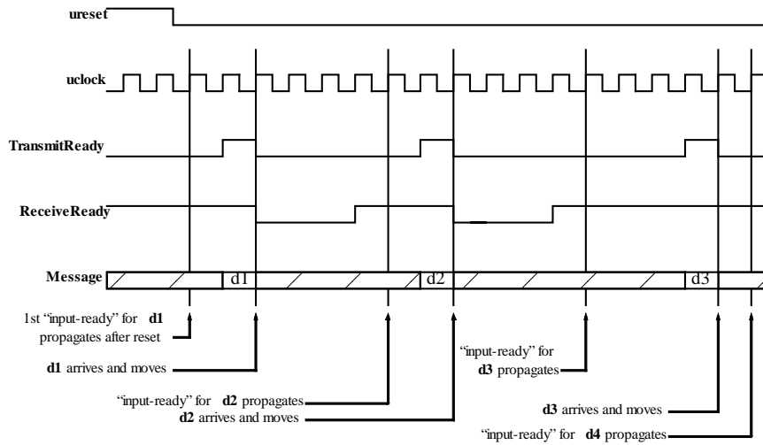
Figure 5.3 SceMiMessageInPort handshake waveforms with input-ready propagation
