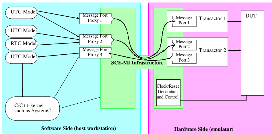
Figure 4.2 High-level view of run-time components
