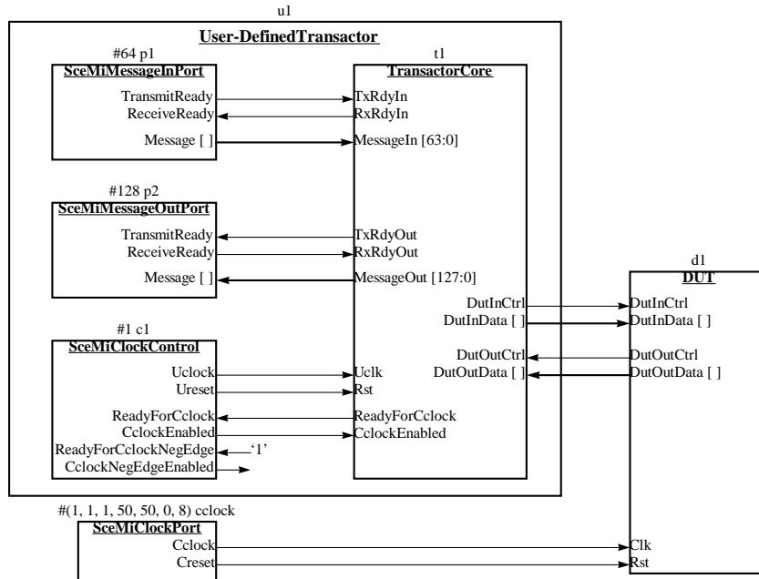
Figure A.1 Connection of SCE-MI macros on hardware side to transactor and DUT
