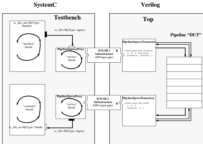
Figure A.7 DPI Interfacing between a SystemC TB and a SystemVerilog DUT
