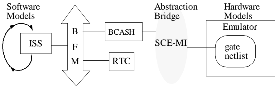
Figure 3.1 Using the SCE-MI as an abstraction bridge
