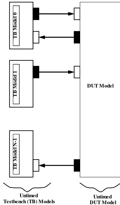
Figure 4.3 Untimed software testbench and DUT models
