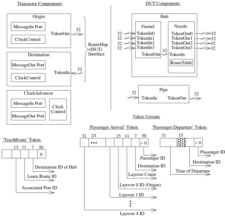
Figure A.5 DUT and transactor components
