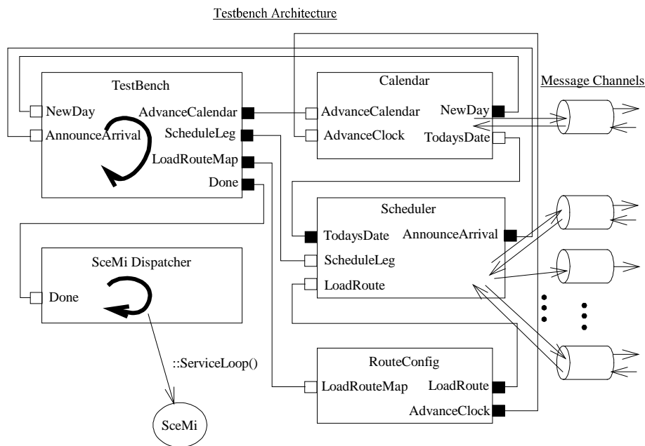
Figure A.6 Interconnect of SystemC models
