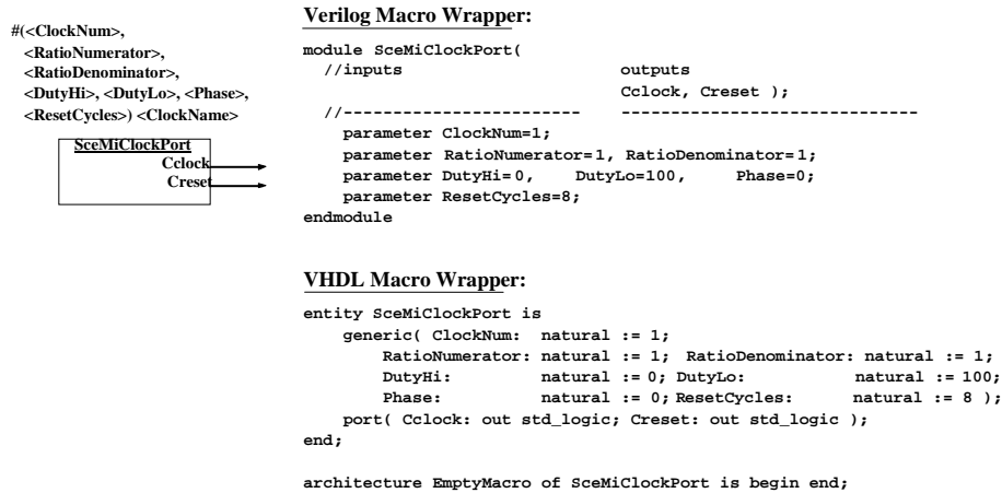
Figure 5.5 SceMiClockPort macro
