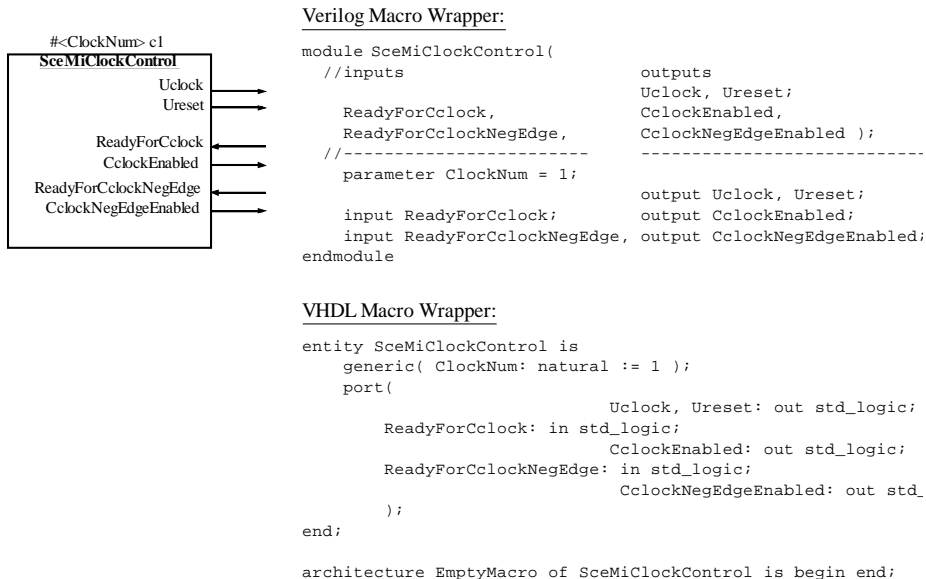
Figure 5.7 SceMiClockControl macro
