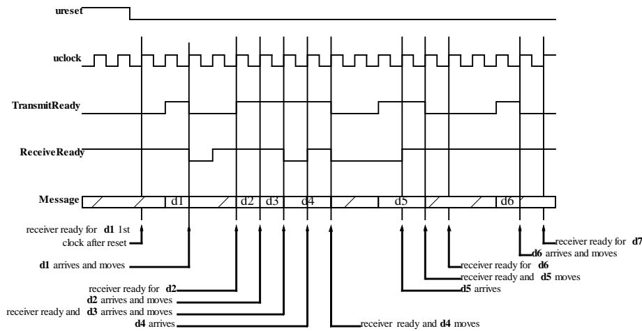
Figure 5.1 Dual-ready handshake protocol
