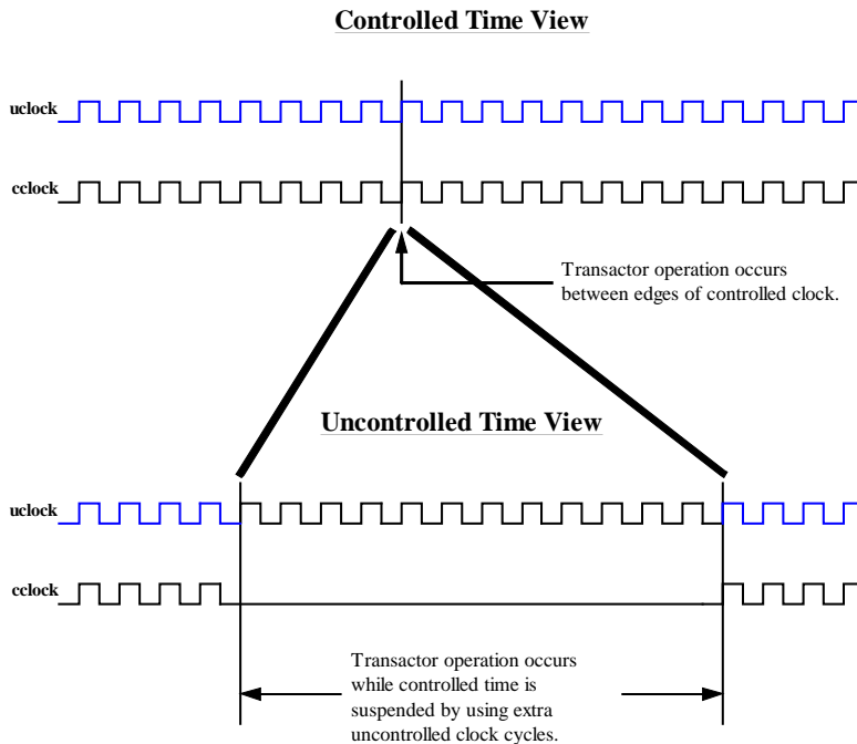
Figure 4.5 Controlled and uncontrolled time views
