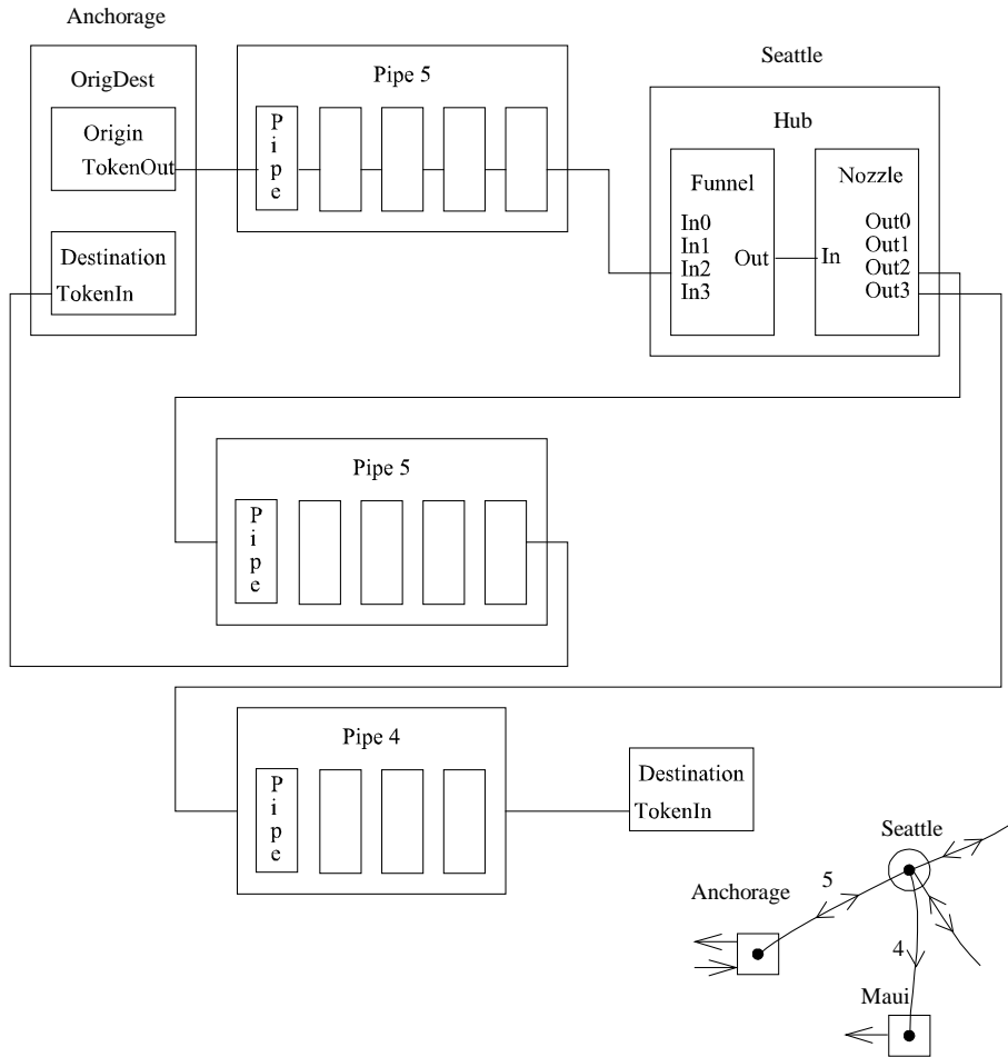
Figure A.4 DUT and transactor interconnect
