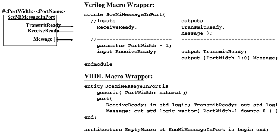
Figure 5.2 SceMiMessageInPort macro
