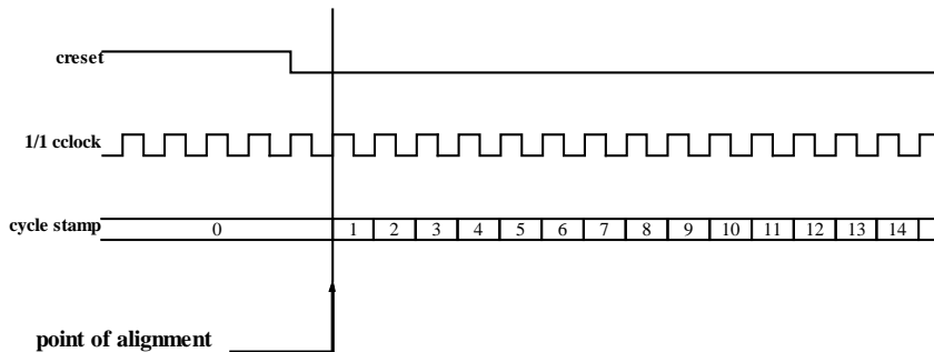
Figure 5.10 Cycle Stamps
