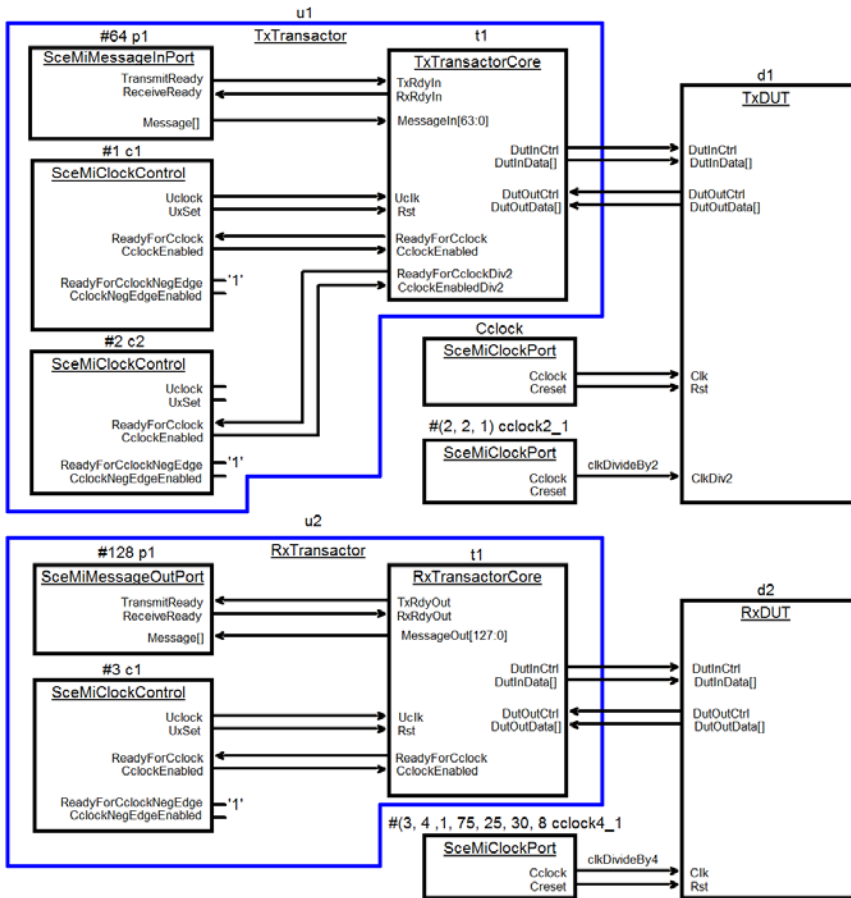
Figure D.1 Multi-clock, multi-transactor example
