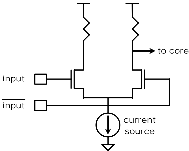
Figure 4.6 – Half-differential Receiver
