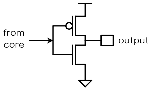
Figure 4.8 – Single-ended Driver
