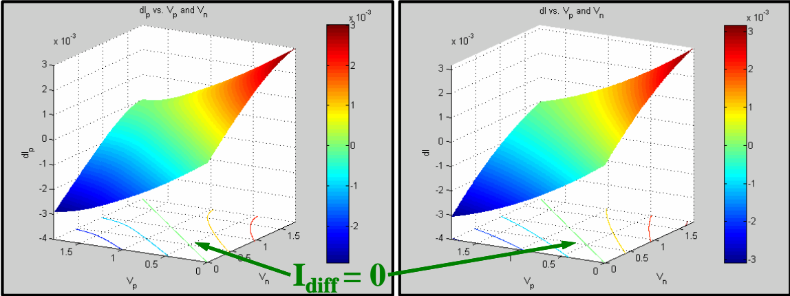
Figure 4.16 – Differential Current Plot of Output Current versus P and N Voltage
