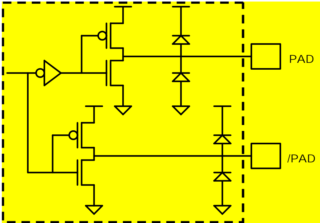
Figure 3.1: Pseudo-Differential Buffer
