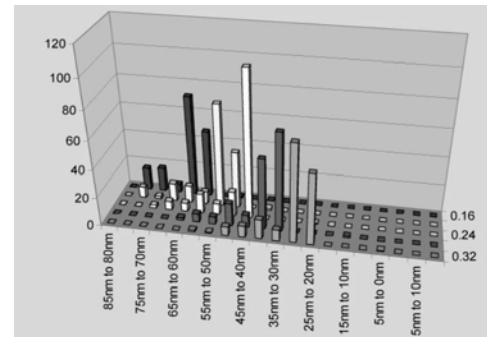
Figure 5.2: Layout Process Signature (Focus,Dose)
