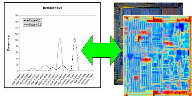
Figure 5.3: Layout Process Signature (Full-Chip Map)
