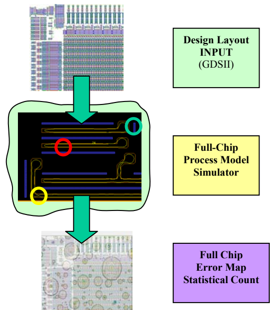
Figure 2: DFM Functional Building Block
