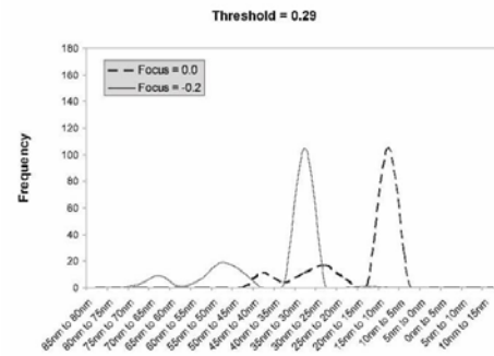
Figure 5.1: Layout Process Signature (Focus)
