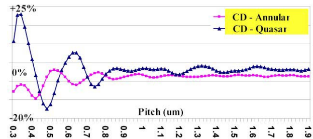
Figure 4: Forbidden Pitches for Annular and Quasar
