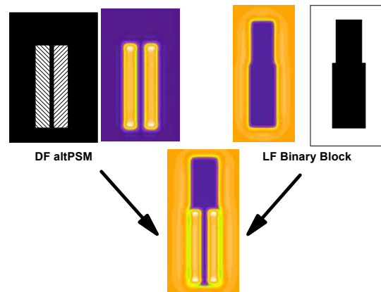
Figure 6 Double exposure altPSM
