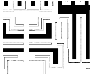
Figure 8 Sraf-enhanced layout showing local sraf conflicts
