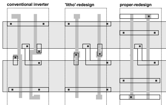
Figure 15. Optimization at design (right) and layout level (center)
