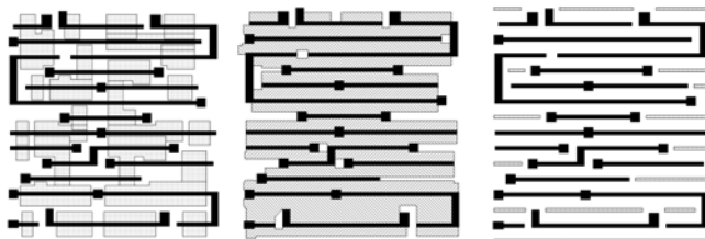
Figure 16. Latch cell designed with RDR (left) is simultaneously altPSM optimized (center) and OAI-attPSM-SRAF optimized (right).
