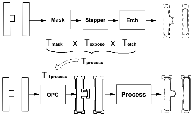
Figure 2, Optical proximity correction
