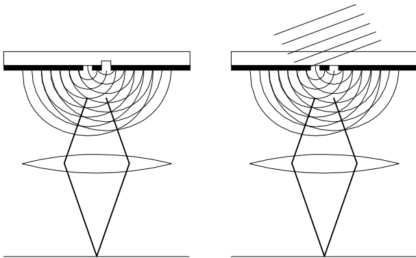
Figure 4 , altPSM (left) and OAI (right) produce 2-beam imaging
