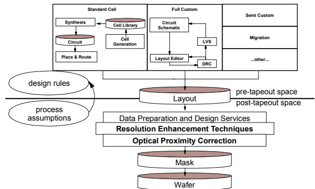
Figure 3, diagram of conventional, DRC-enabled layout flow
