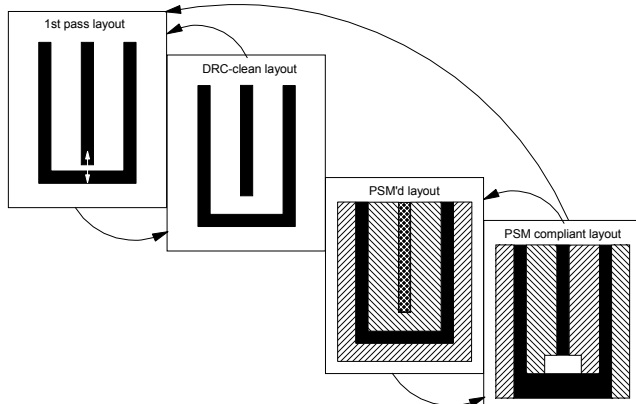
Figure 11. Example of cell level RET-embedded layout flow
