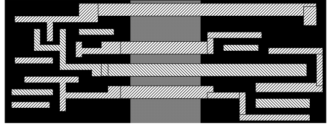
Figure 13. Illustration of challenges for RET-aware routers.
