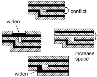
Figure 7 Sample layout conflict (top) and possible solutions
