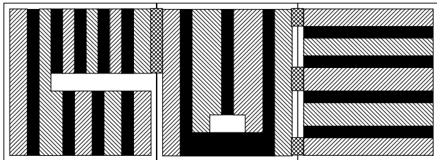
Figure 12. 3 phase-shifted cells with placement-induced conflicts.
