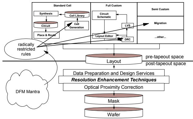
Figure 14. Flow based on 'radically restricted design rules'.
