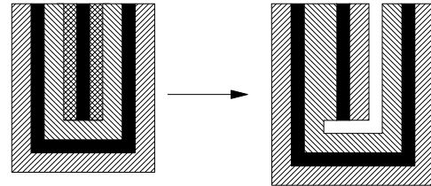
Figure 9 Simple layout forcing complex design rule
