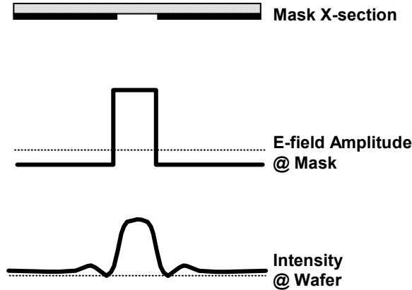
Figure 1, Principle of attenuated phase shifted mask (attPSM)
