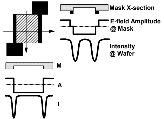
Figure 5 Principle of altPSM
