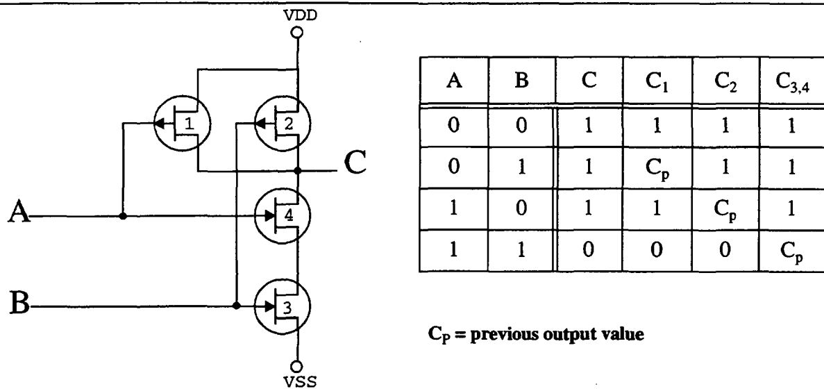
Figure 7: CMOS implementation of a NAND gate.
