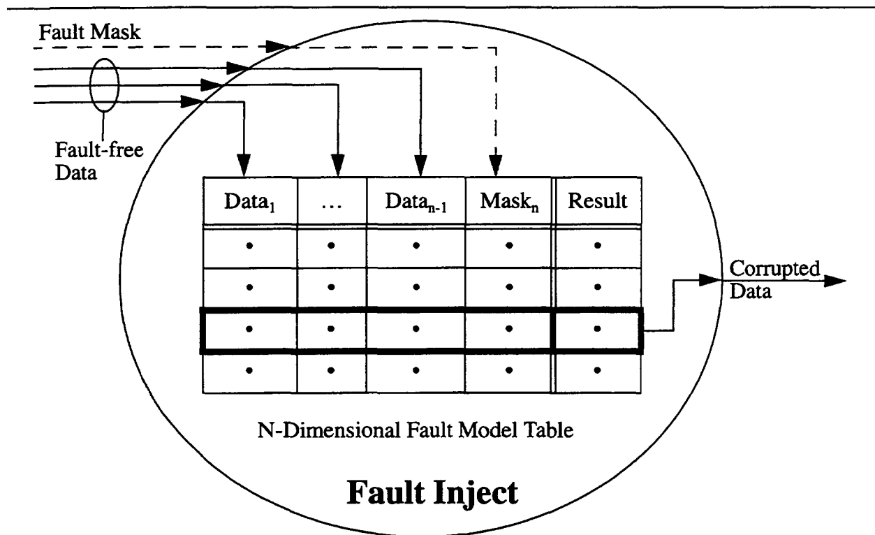
Figure 4: Concurrent procedure call that performs the data corruption.
