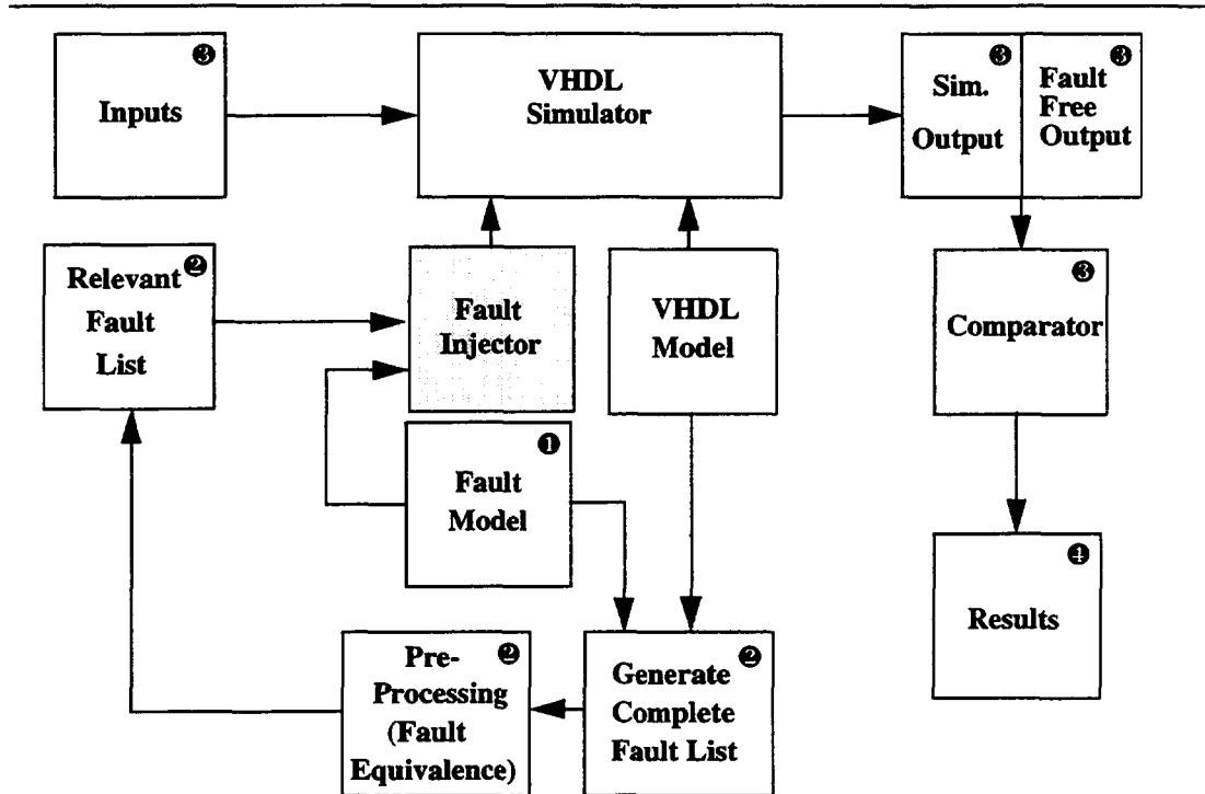
Figure 1: Structure of a simulator-independent VHDL fault simulator.
